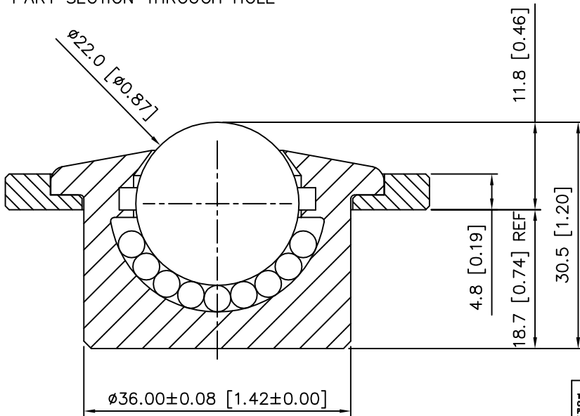
PART SECTION THROUGH HOLE
